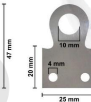
KRM-K-PDE-F-M40
